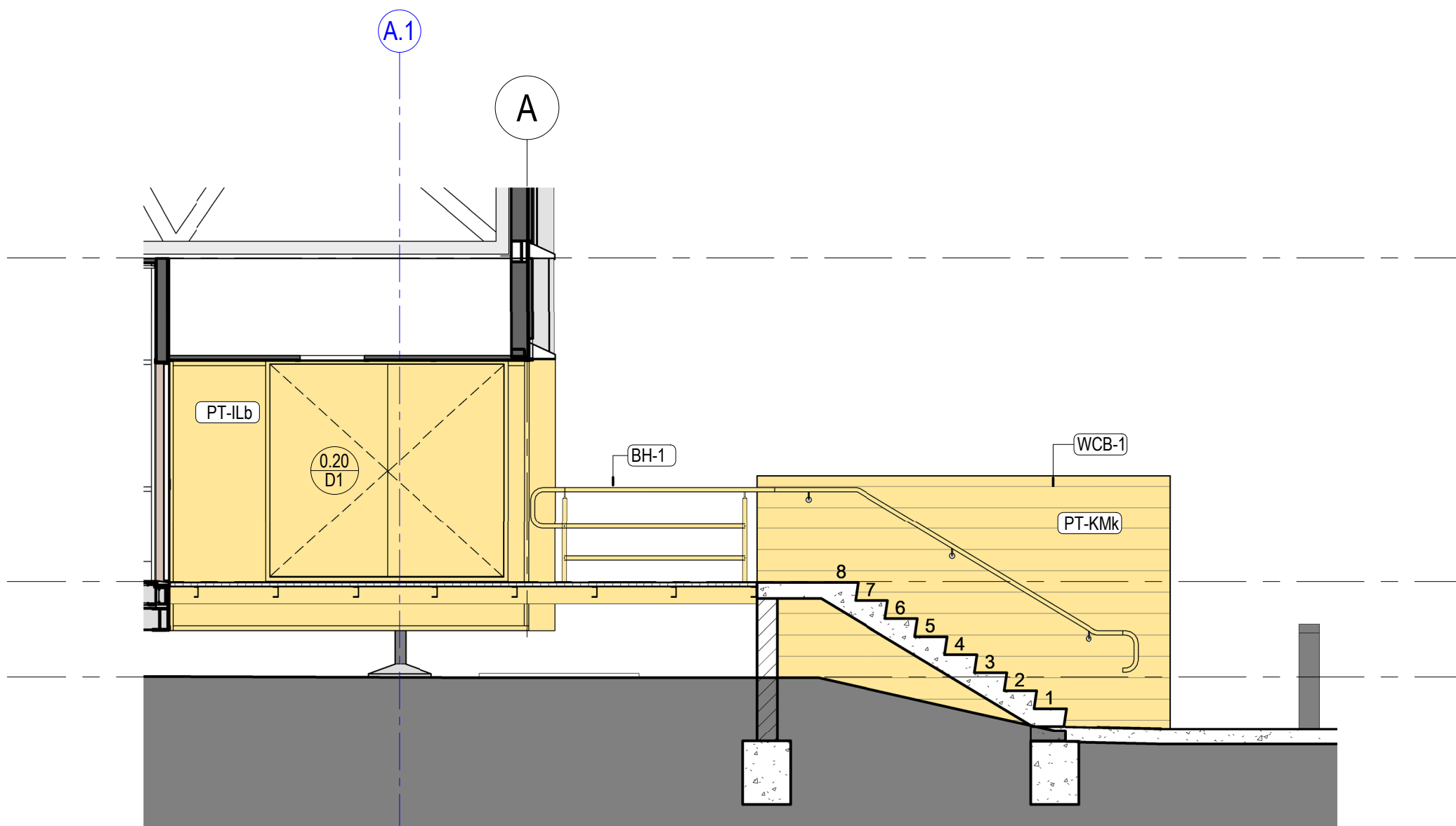
7 Stair 2 - Section 2 1:50
