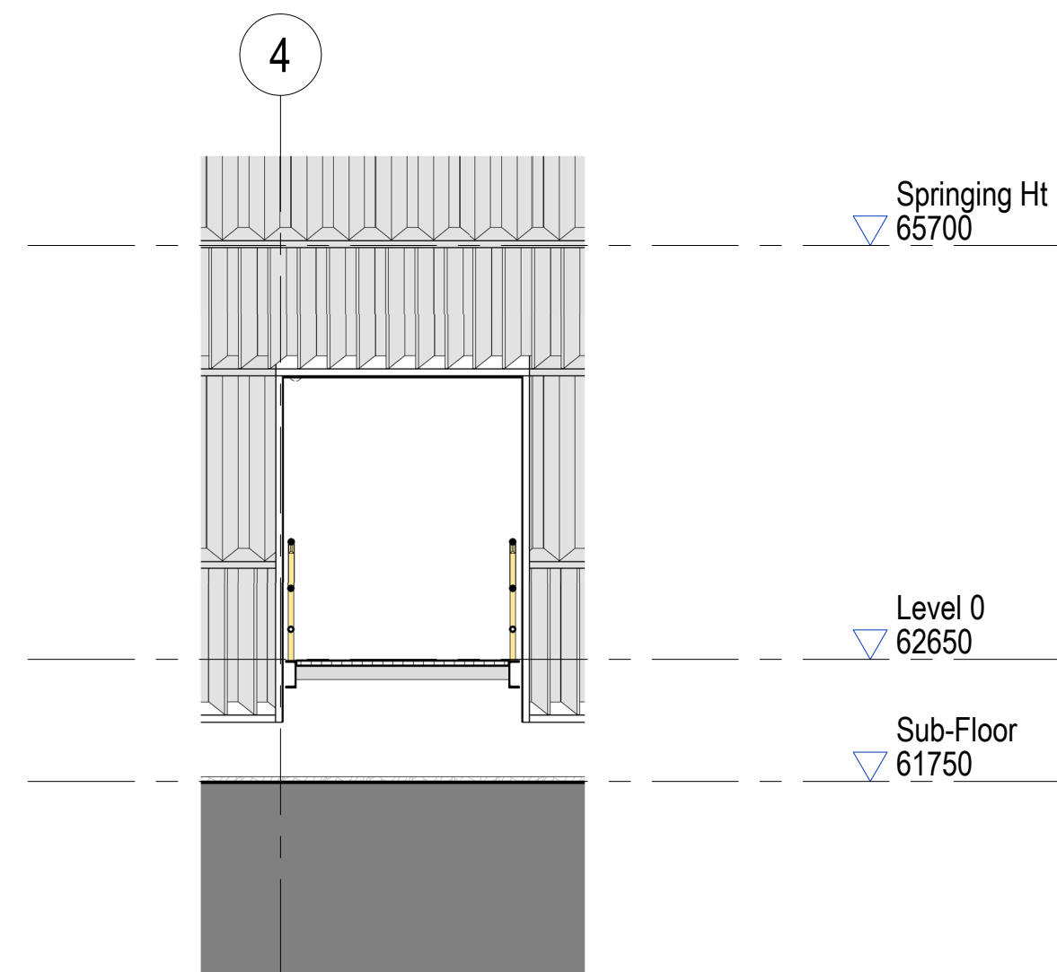
9 Stair 2 - Section 4 1:50
