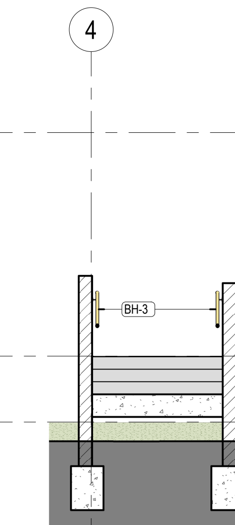
8 Stair 2 - Section 3 1:50
